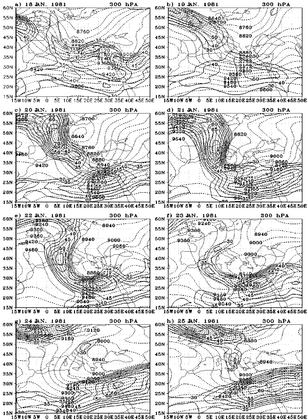
Fig. 5. 300 hPa geopotential contours every 60 gpm intervals dashed and isotachs solid those \geq 30 m/s every for 1200 UTC 18-25 January 1981.
