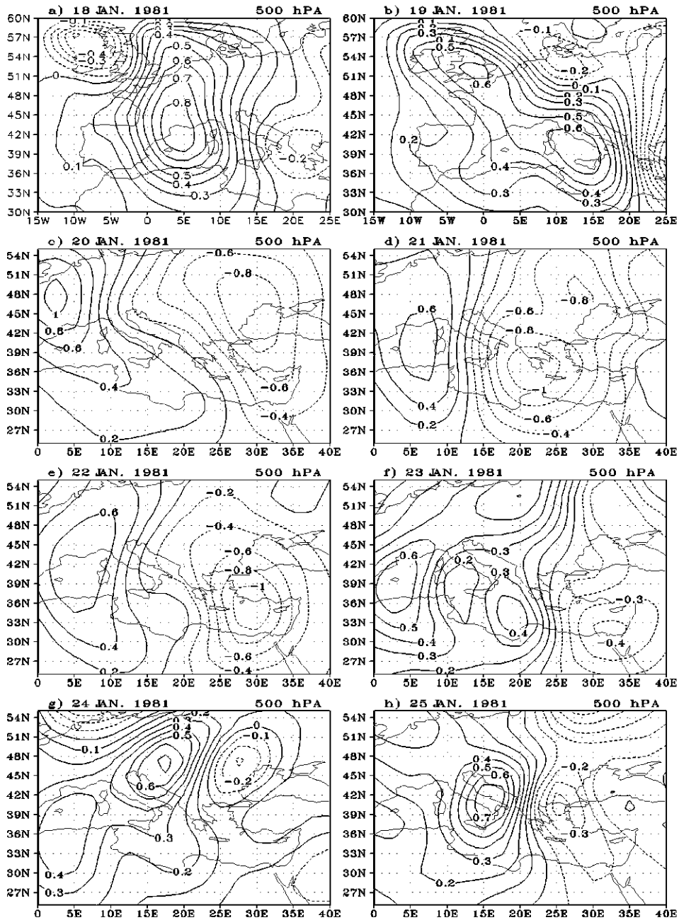
Fig. 8. Vertical motion analysis at 500 hPa contours every 0.1 \text{ Pa S}^{-1} , solid lines denote positive values dashed lines denote negative values for 1200 UTC 18-25 January 1981.
