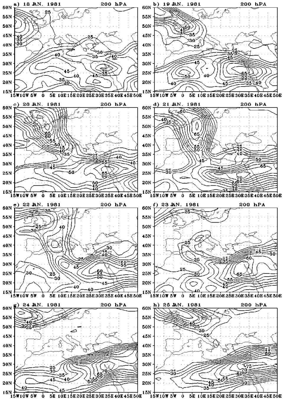
Fig. 4. Isotachs at 200 hPa those \geq 25 m/s, every 5 m/s, for 1200 UTC 18-25 January 1981.
