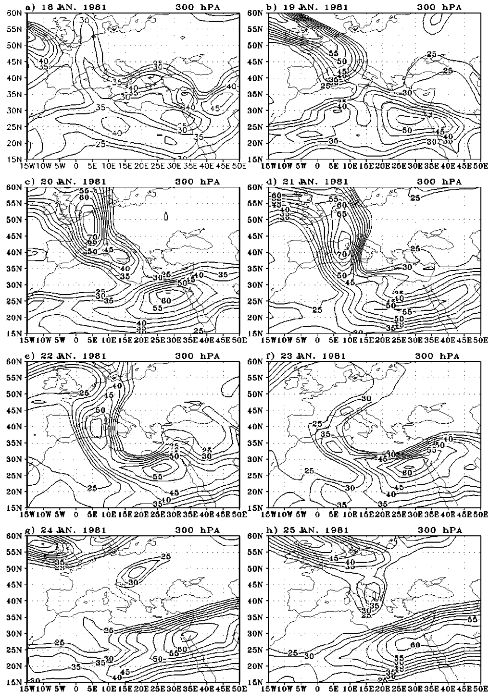
Fig. 3. Isotachs at 300 hPa, those \geq 25 m/s, every 5 m/s, for 1200 UTC 18-25 January 1981.
