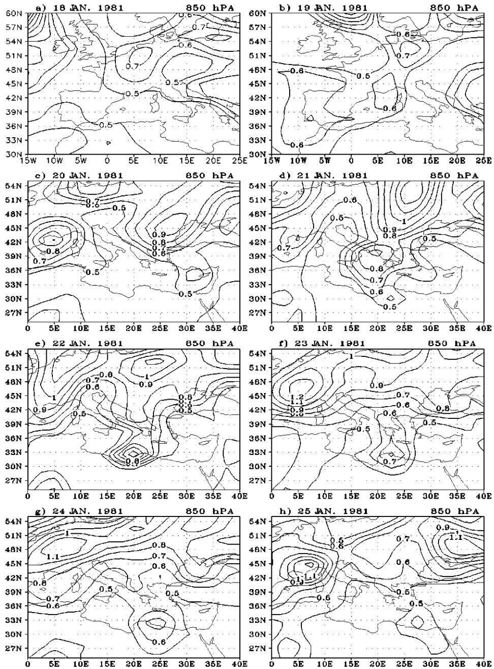
Fig. 11. Ertel's positive potential vorticity analysis at 850 hPa, \geq 0.5 PVU, contours every 0.1 PVU for 1200 UTC 18-25 January 1981.
