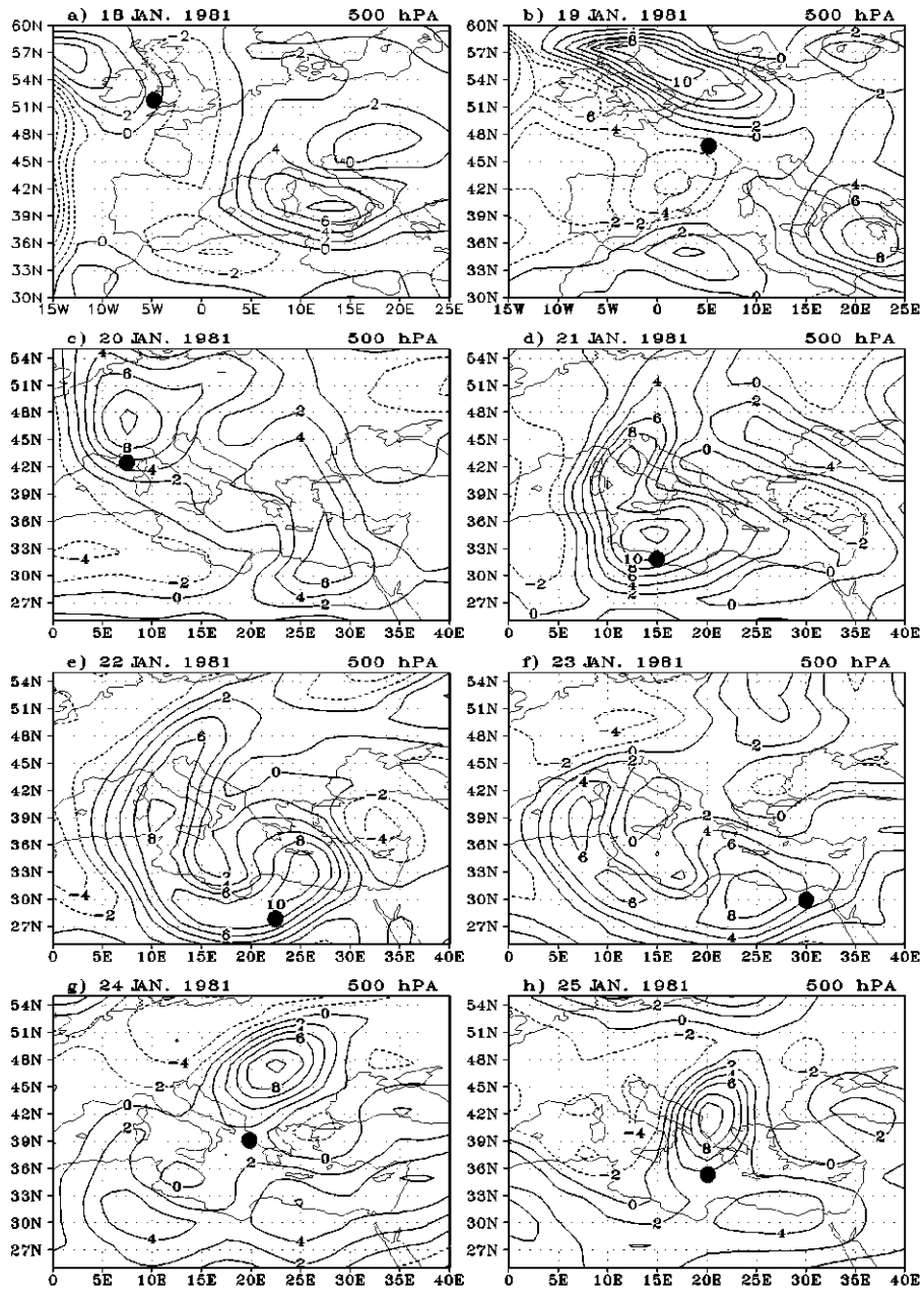
Fig. 6. Relative vorticity analysis at 500 hPa, contours every 2.0 \times 10^4 \text{ s}^{-1} , solid lines denote positive values, dashed lines denote negative values. Also indicated are the centers of 500 hPa maximum absolute vorticity advection (filled circle) for 1200 UTC 18-25 January 1981.
