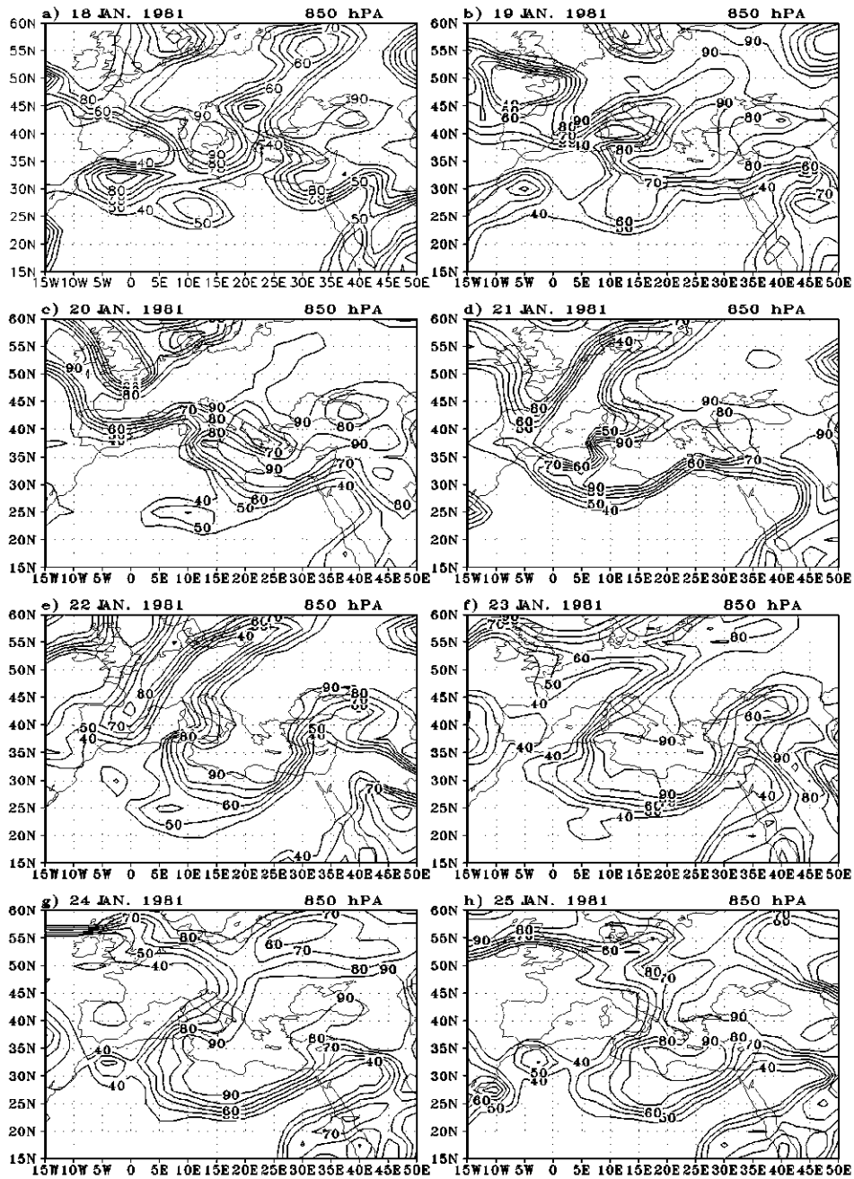
Fig. 9. Relative humidity objective analysis at 850 hPa, that \geq 40\% isopleths every 10% for 1200 UTC 18-25 January 1981.
