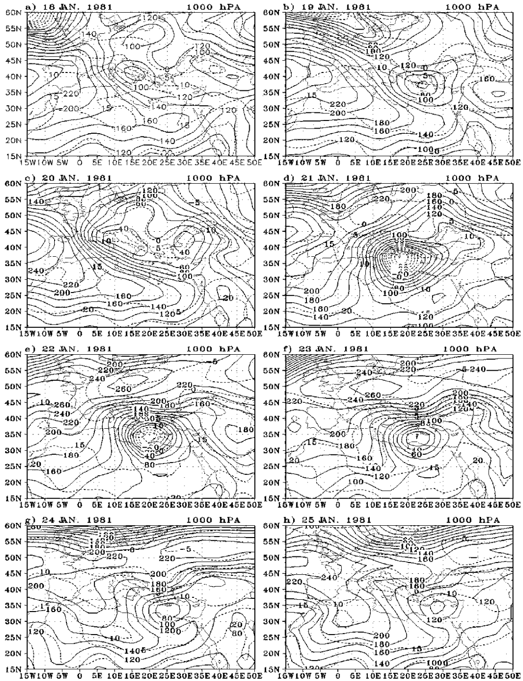
Fig. 1. The 1000 hPa geopotential contour every 20 m intervals (solid) and temperature dashed every 5°C for 1200 UTC 18-25 January 1981.
